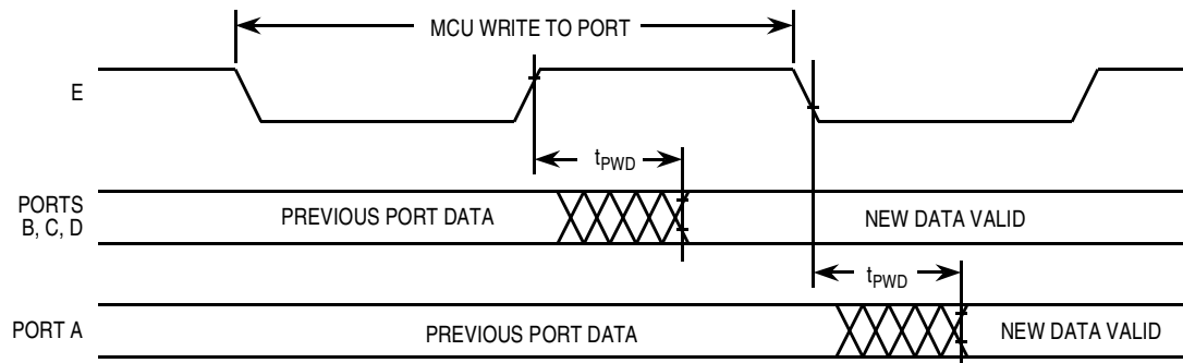
Figure 11-8. Port Write Timing Diagram
