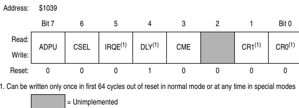
Figure 5-2. System Configuration Options Register (OPTION)
